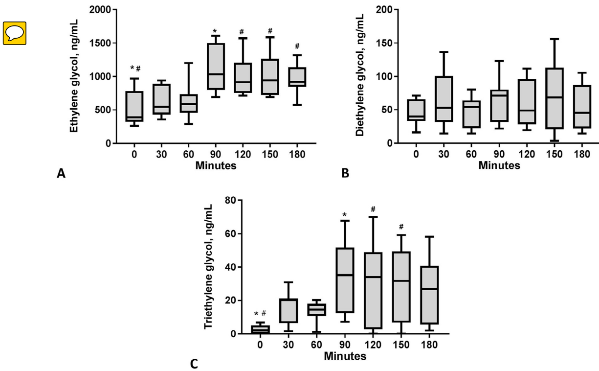
Figure 2. Median and total ranges of blood levels of A , EG; B , DEG; and C , TEG after ingestions of 17 grams of PEG 3350 (* P < .01, # P < .05).
