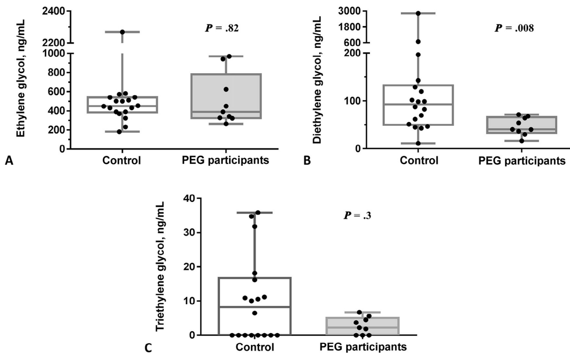
Figure 1. Baseline median and total ranges of blood levels of A , EG; B , DEG; and C , TEG of controls and study participants.
