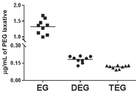
Figure 3. Calculated amounts of EG, DEG, and TEG in PEG 3350 suspended in 8 oz (237 mL) of water. Bar indicates mean.
