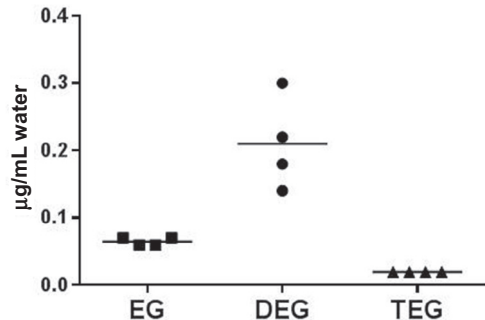
Figure 4. Amounts of EG, DEG, and TEG found in public water supply. Bar indicates mean.
